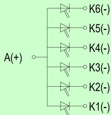
BACKLIGHT CIRCUIT
