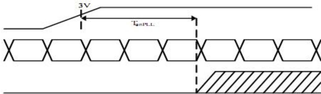
LVDS timing(2)
