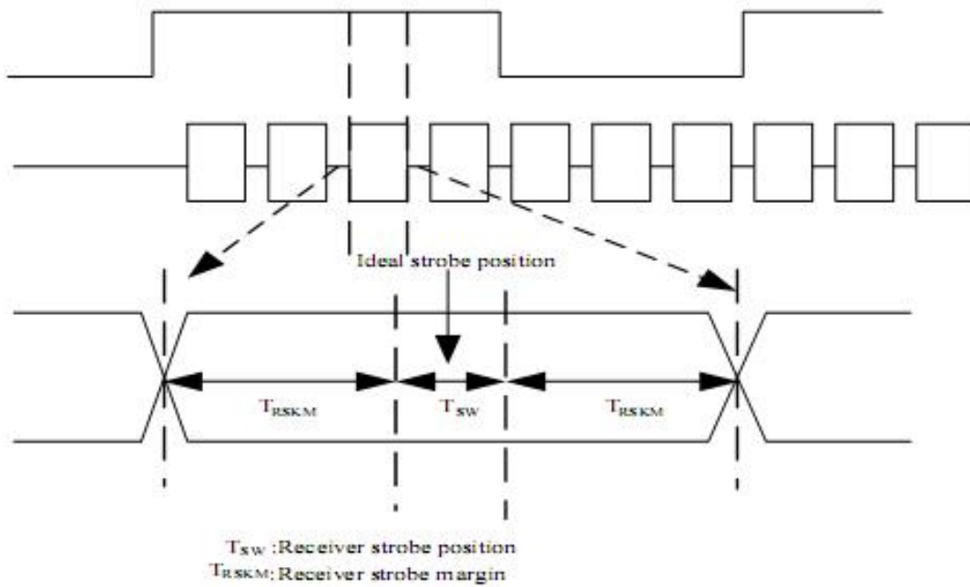
LVDS timing(2)
