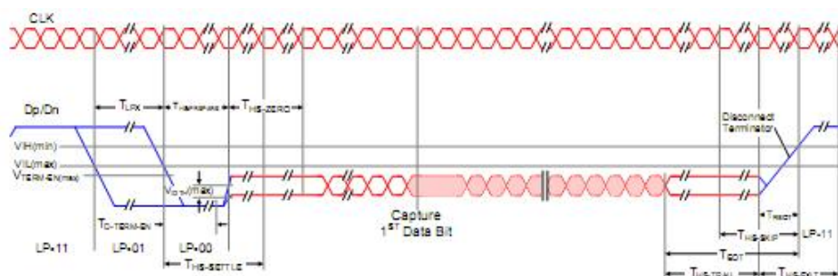
Figure 1 : High-Speed Data Transmission in Bursts
