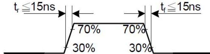
8080 Parallel Interface Characteristics
